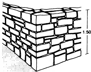
③ Squared random rubble uncoursed walling
